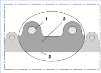
Vacuum truck hose, extremely heavy duty
