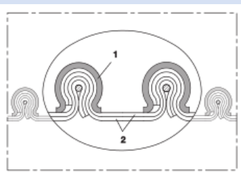
High-temperature hose, clamp profile hose (clip hose), (up to +932 °F)
