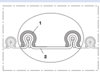
Electrically conductive clamp profile hose (clip hose), (up to +410 °F)
